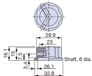
Dimensions (mm)
