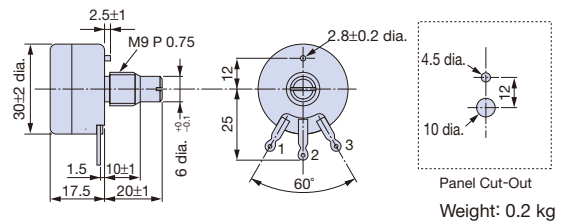
Dimensions (mm)
