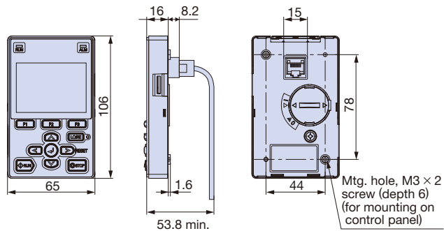
Dimensions (mm)
