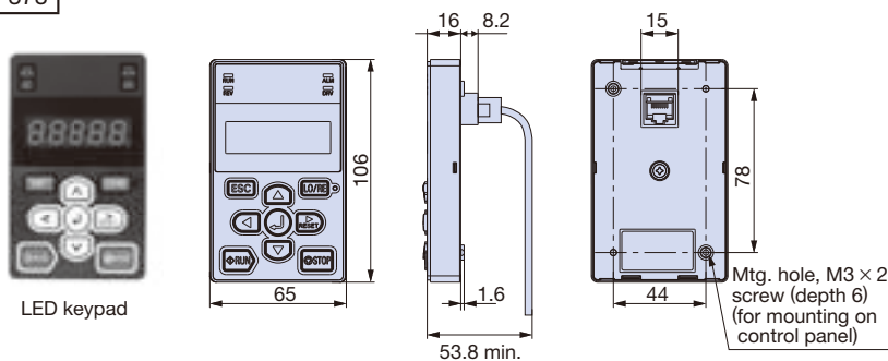
Dimensions (mm)
