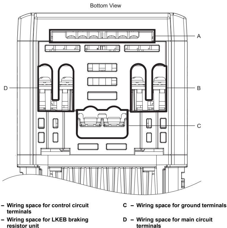
Figure 15 Wiring Spaces
