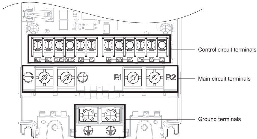
Figure 16 CDBR Wiring Terminals
