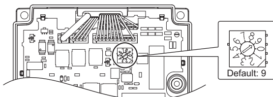
Figure 26 CDBR Voltage Activation Level, Rotary Switch (S3)
